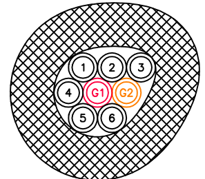
(6) 3/8" PRODUCT & (2) 3/8" GLYCOL O.D. 3"
