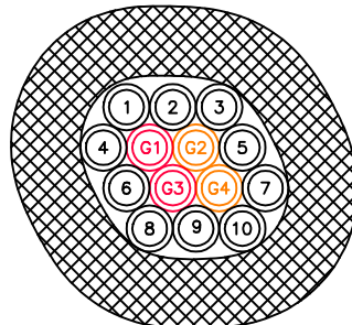
(10) 3/8" PRODUCT & (4) 3/8" GLYCOL O.D. 3-3/4"
