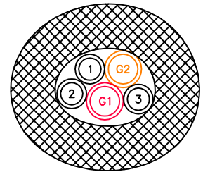
(3) 3/8" PRODUCT & (2) 1/2" GLYCOL O.D. 3-1/4"
