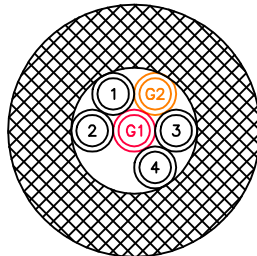
(4) 3/8" PRODUCT & (2) 3/8" GLYCOL O.D. 3"
