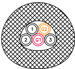
(3) 3/8" PRODUCT & (2) 3/8" GLYCOL O.D. 2-3/4"
