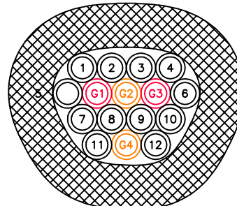
(12) 3/8" PRODUCT & (4) 3/8" GLYCOL O.D. 3-3/4"
