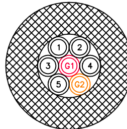
(5) 3/8" PRODUCT & (2) 3/8" GLYCOL O.D. 3"
