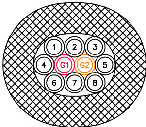
(8) 3/8" PRODUCT & (2) 3/8" GLYCOL O.D. 3-3/8"
